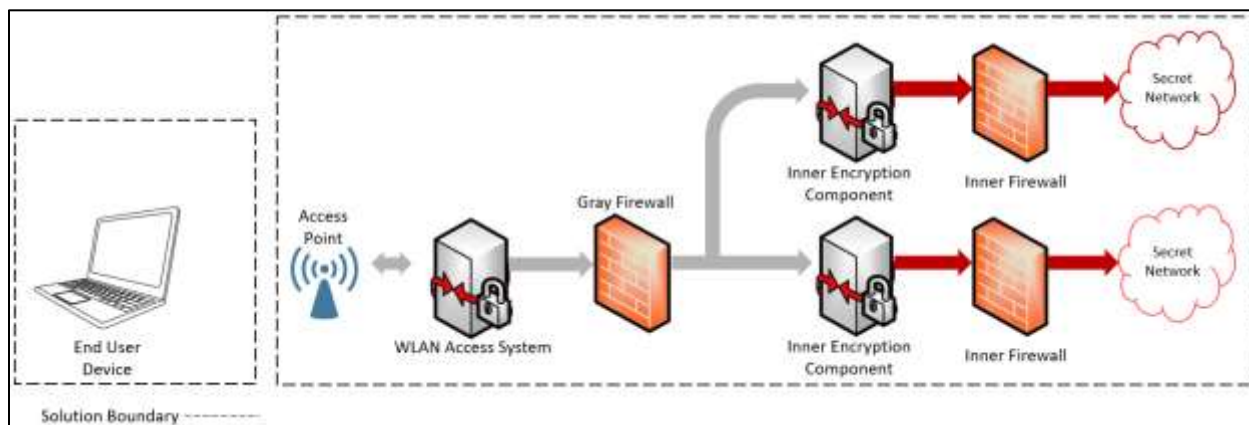
Figure 3. Campus WLAN Solution for Two Networks of the Same Classification Level
