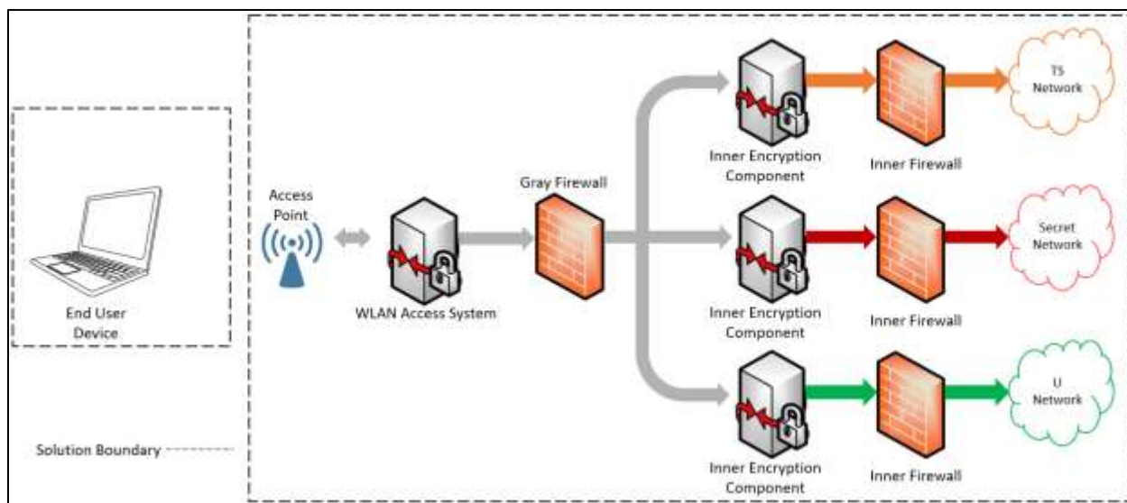
Figure 4. Campus WLAN Solution for Networks Operating at Different Classification Levels
