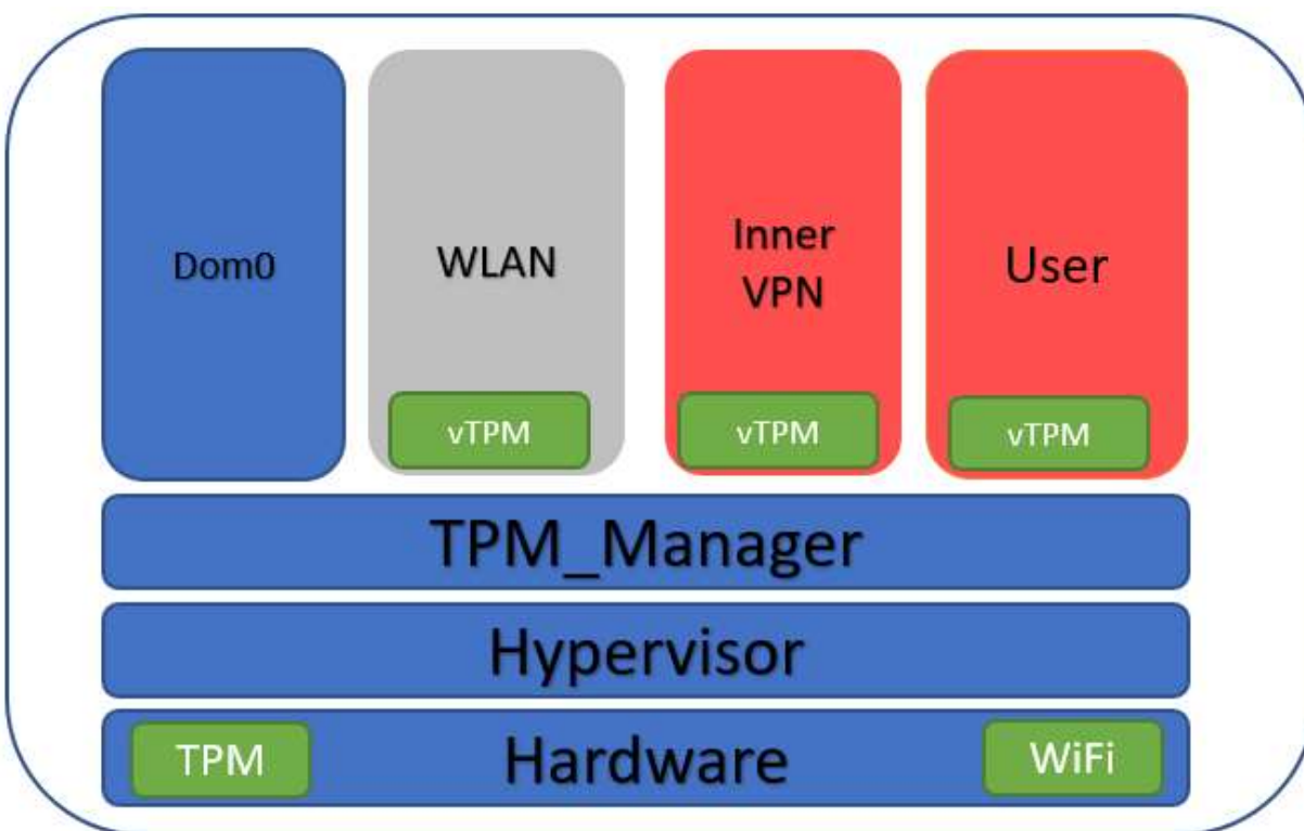
Figure 8. Enhanced Software Virtualization Architecture
