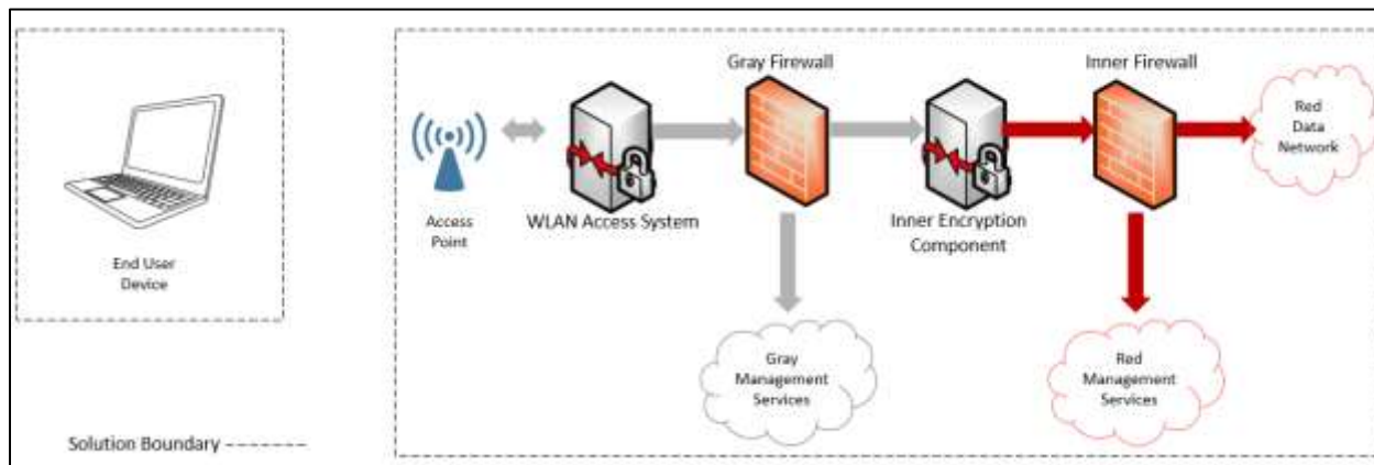
Figure 2. Campus WLAN Single Classification Implementation
