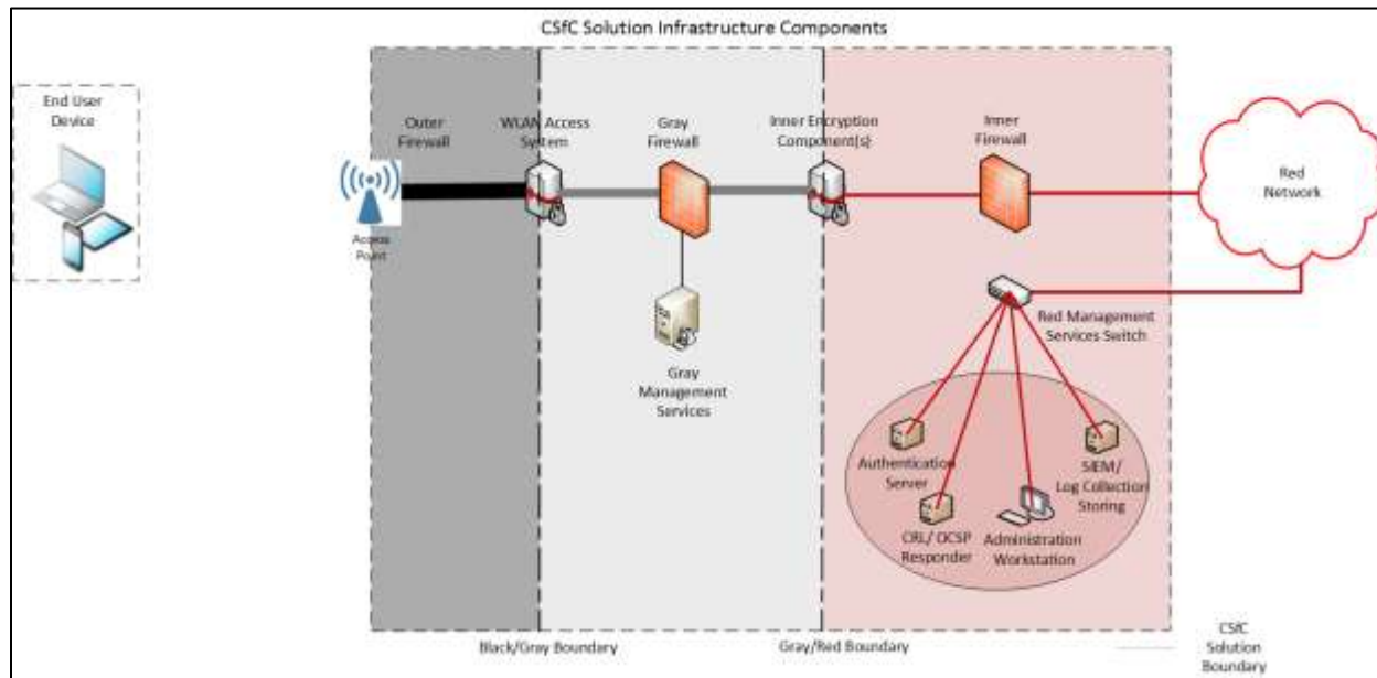
Figure 6. Overview of Red Management Services
