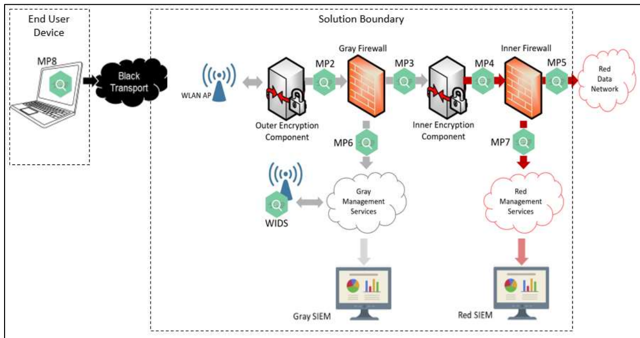
Figure 9. Campus WLAN Continuous Monitoring Points
